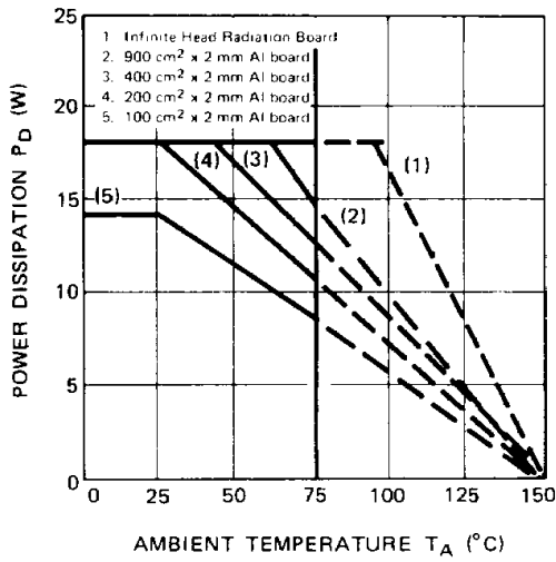
Fig. 9 – POWER DERATING CURVE (MB3732)
