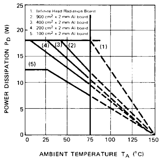
Fig. 10 – POWER DERATING CURVE (MB3734)
