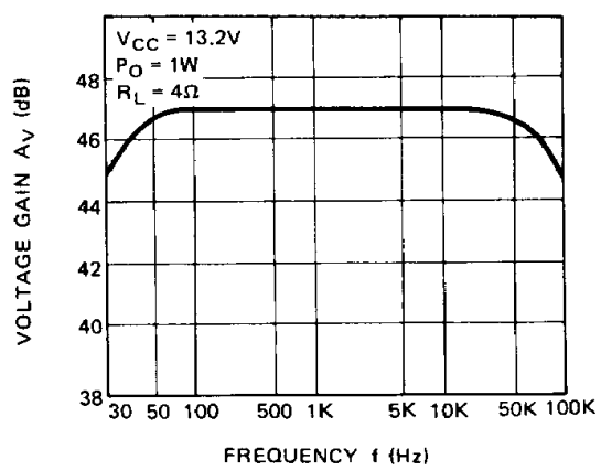
Fig. 8 – VOLTAGE GAIN vs. FREQUENCY
