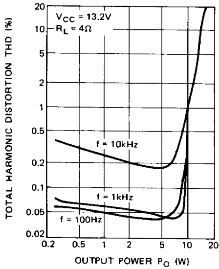
Fig. 5 – TOTAL HARMONIC DISTORTION vs. OUTPUT POWER
