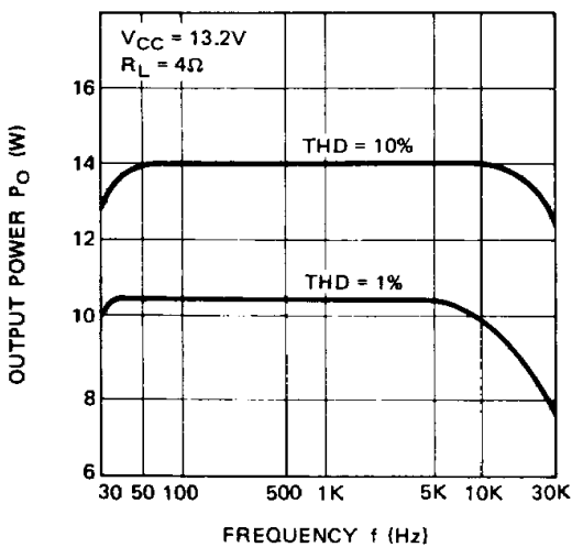
Fig. 7 – OUTPUT POWER vs. FREQUENCY
