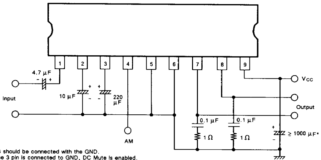
Fig. 4 – MB3734 TEST CIRCUIT
