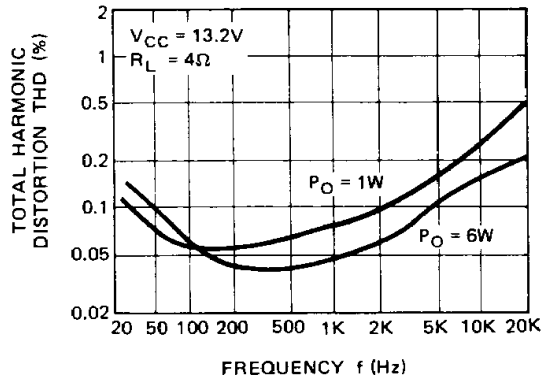
Fig. 6 – TOTAL HARMONIC DISTORTION vs. FREQUENCY
