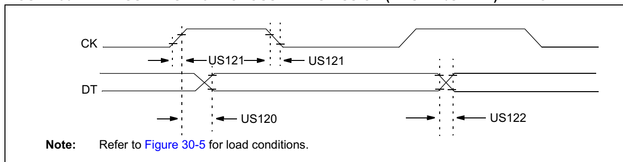
FIGURE 30-14: USART SYNCHRONOUS TRANSMISSION (MASTER/S�AVE) TIMING
