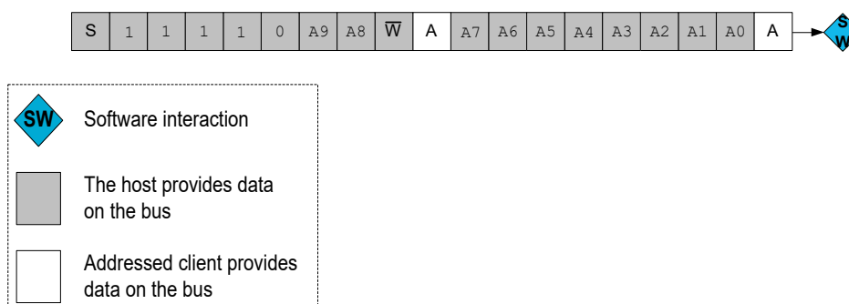
Figure 29-9. 10-Bit Address Transmission
