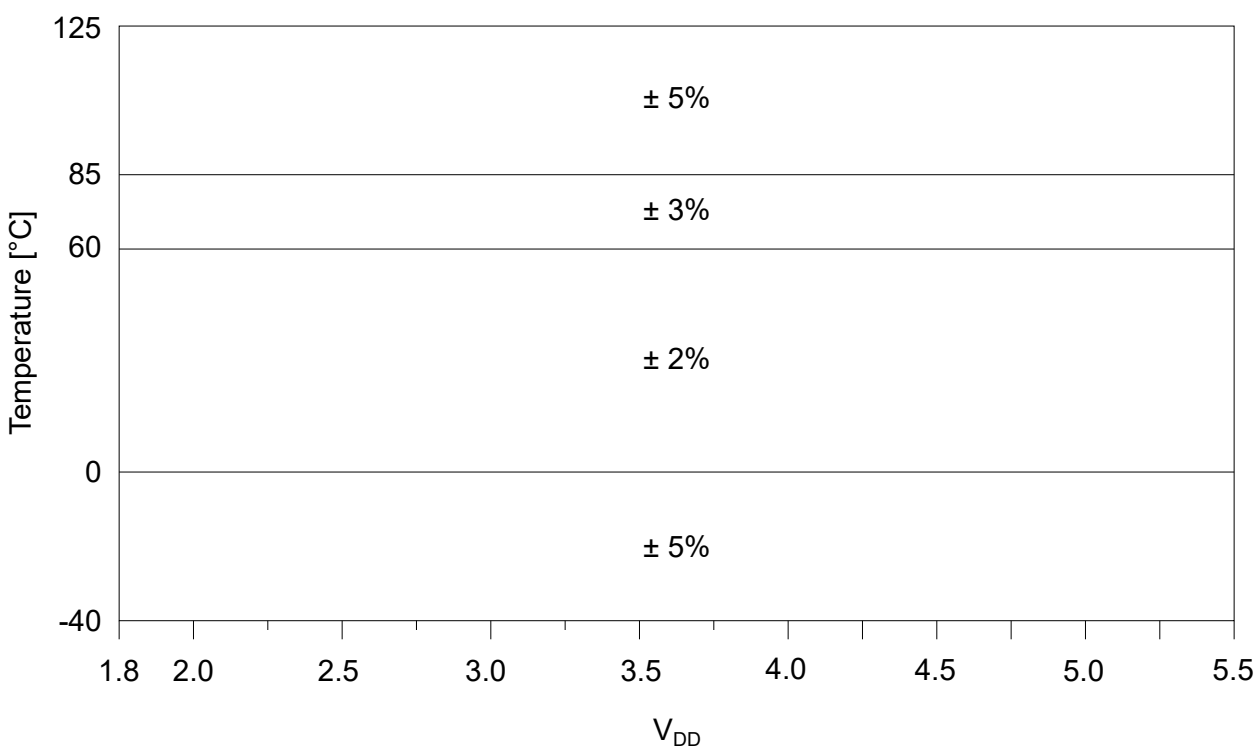
Figure 38-2. Precision Calibrated OSCHF (4 MHz) Frequency Accuracy Over Device V_{DD} and Temperature
