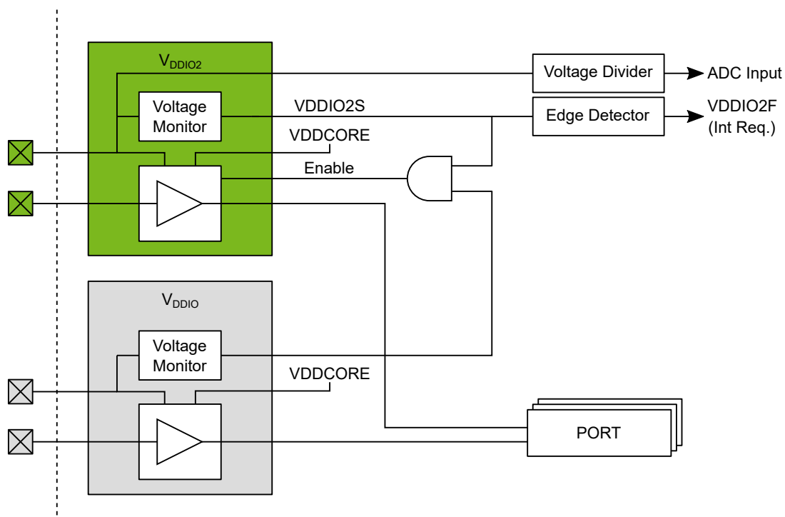
Figure 19-1. MVIO Block Diagram
