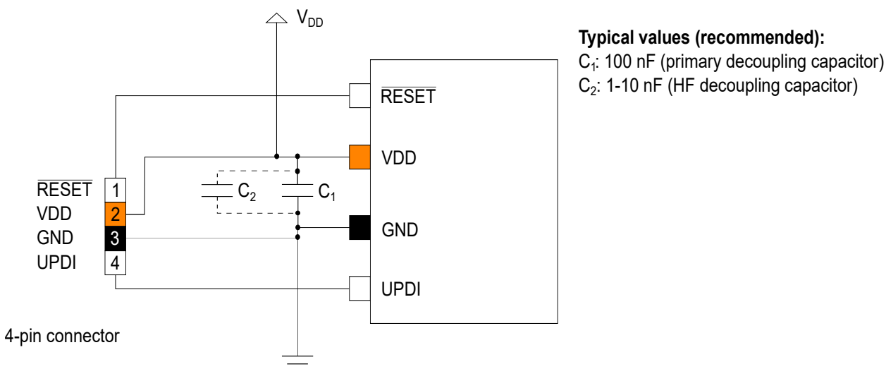
Figure 4-6. Recommended UPDI Programming Circuit Schematic
