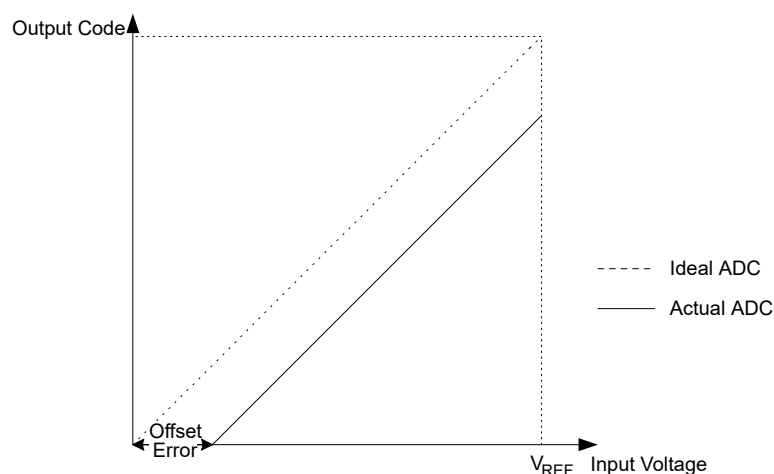
Figure 6-1. Offset Error
