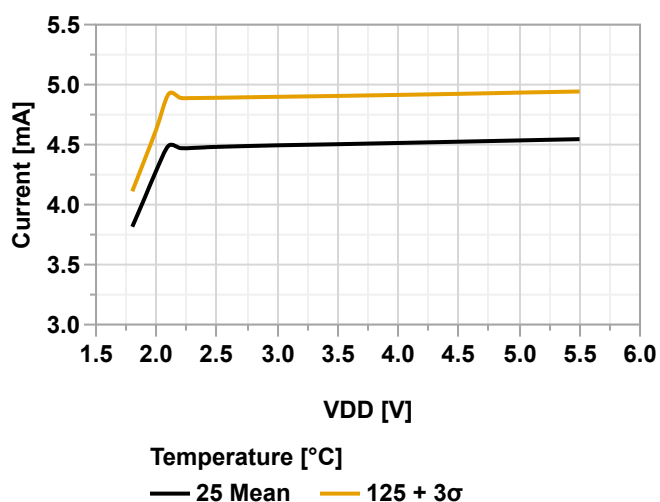
Figure 39-4. Active Power Consumption vs. V_{DD} (MCLKCTRLA.CLKSEL = OSCHF, OSCF = 24 MHz)
