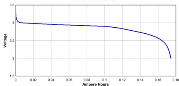
Continuous Discharge Multiple Loads
