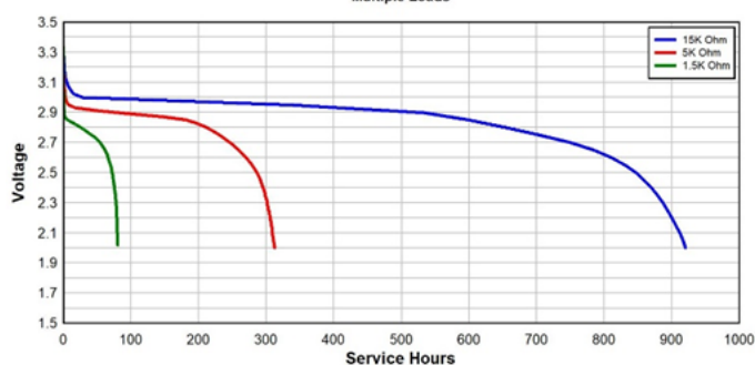
Continuous Discharge Multiple Loads
