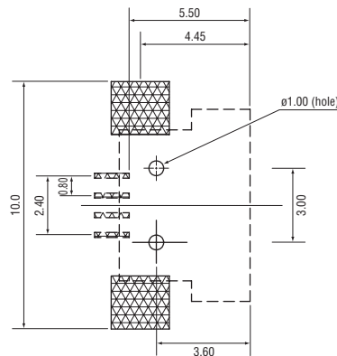
Recommend PCB Layout (tolerance = ±0.05)
