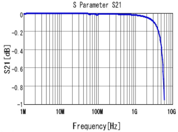
■ GRM3195C1H393JA01 S21 DCOV, 25degC
