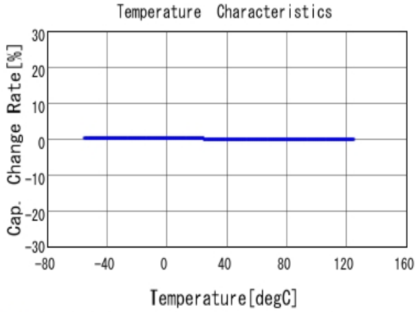
■ GRM3195C1H393JA01 C-Temp. capchange, DCOV, AC1Vrms
