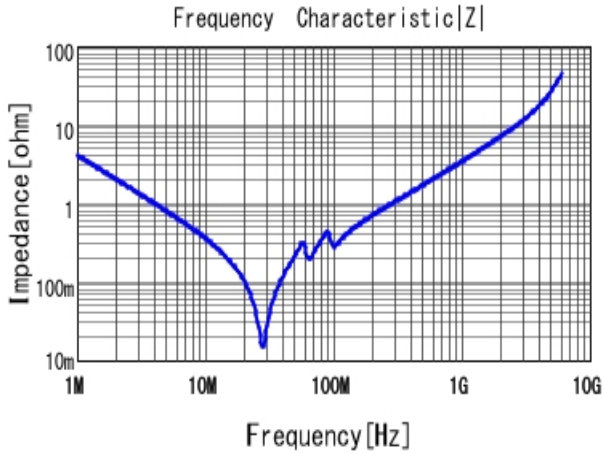
■ GRM3195C1H393JA01 |Z| DCOV, 25degC
