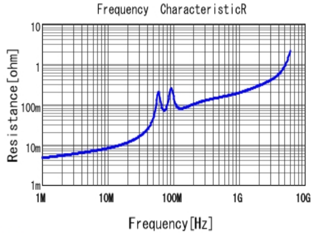
■ GRM3195C1H393JA01 R DCOV, 25degC
