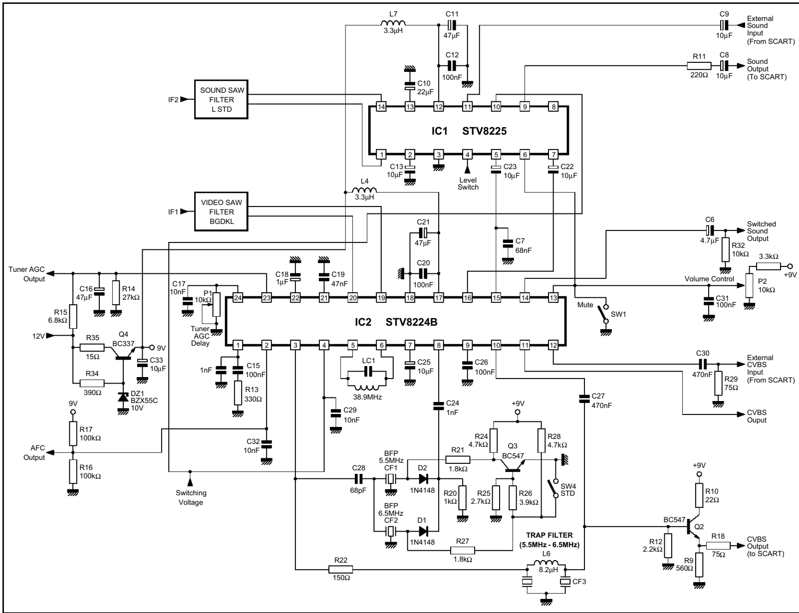
APPLICATION DIAGRAM (B/G/D/K,L) STV8224B - STV8225
