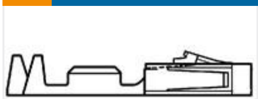
TE Part #1-104480-7 SHORT POINT CONT PLTD SN
