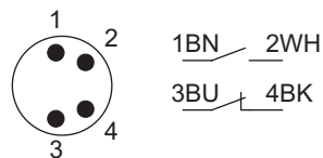
Abb. 7 1 NO + 1 NC (ohne LED)
