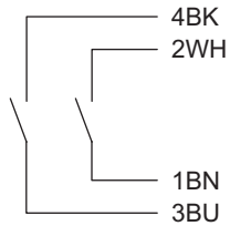
Abb. 1 2 NO (ohne LED)
