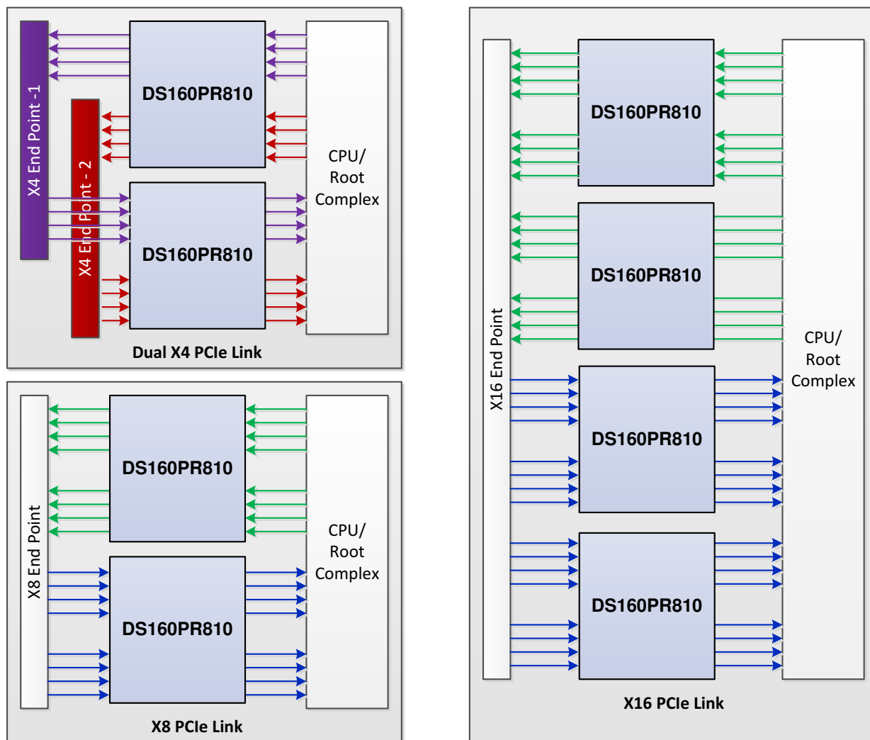
Figure 8-1. PCI Express x4, x8 and x16 use cases using DS160PR810
