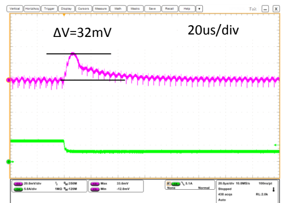
Step Load Transient Response (Vin=5.0V, Vout=1.0V, Clod=400uF, Iout=3A to 6A, 2.5A/us) Trace 3=Vout, 20 mV/div, Trace 4=Iout, 5A/div.
