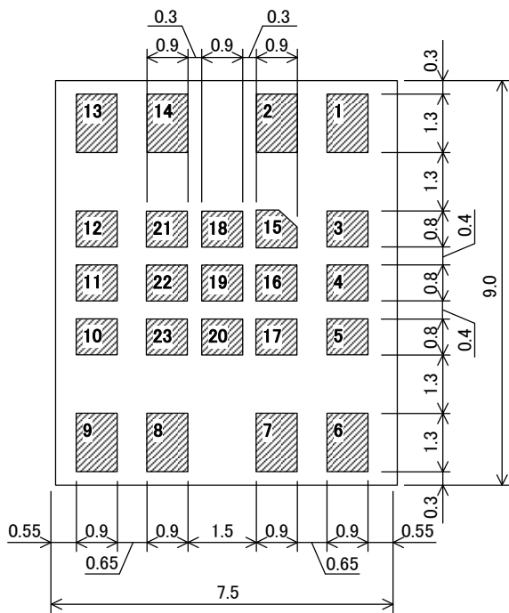
< Bottom View >
