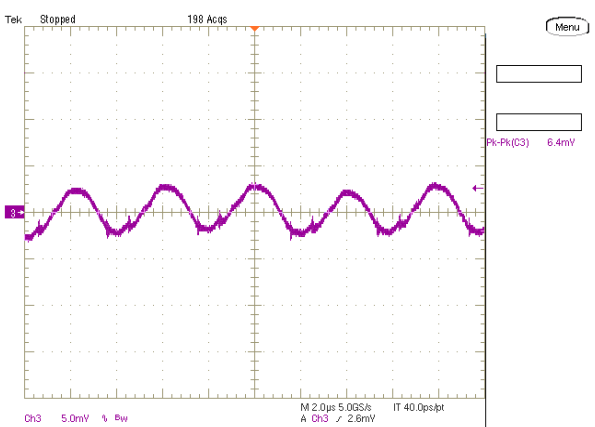
Output Ripple and Noise (Vin=5.0V, Vout=1.0V, Iout=6A, Clod=400uF, ScopeBW=20MHz)
