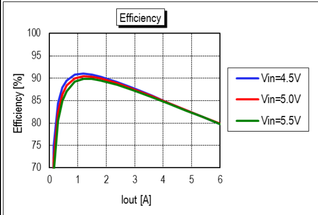
Efficiency vs. Line Voltage and Load Current @ +25degC. (Vout = 0.7V)
