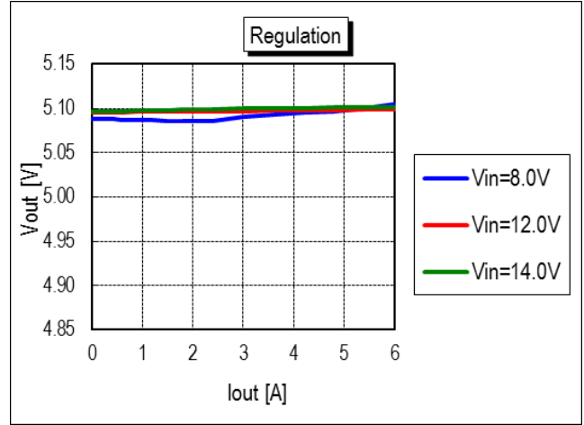
Vout vs. Line Voltage and Load Current @ +25degC. (Vout = 5.0V)
