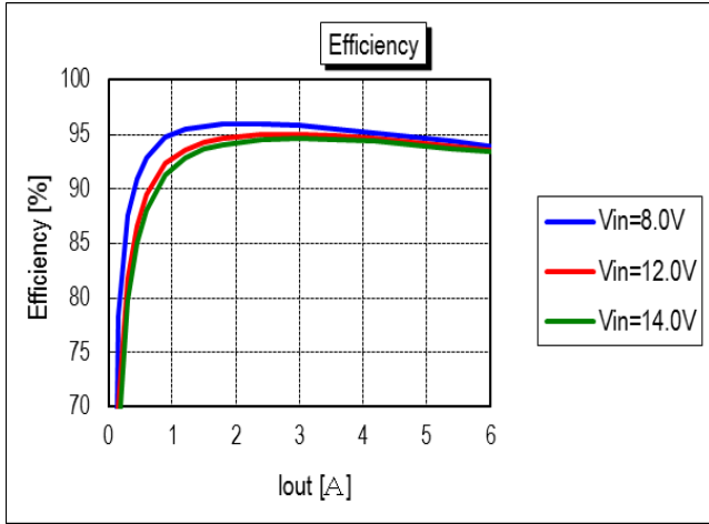
Efficiency vs. Line Voltage and Load Current @ +25degC. (Vout = 3.3V)
