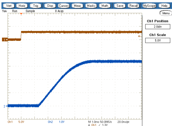
On/Off Enable Delay (Vin=12V, Vout=3.3V, Iout=6A, Cload=400uF) Trace1=Enable, Trace2=Vout, 1 ms/div
