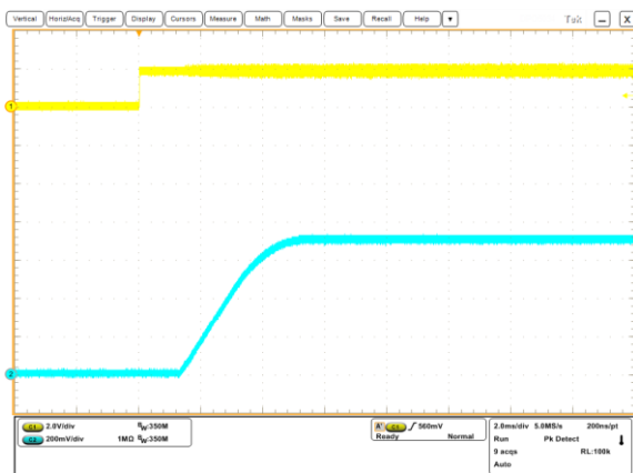
On/Off Enable Delay (Vin=5.0V, Vout=0.7V, Iout=6A, Cload=400uF) Trace1=Enable, Trace2=Vout, 2ms/div
