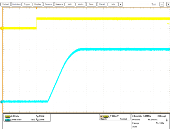
On/Off Enable Delay (Vin=5.0V, Vout=1.0V, Iout=6A, Clod=400uF) Trace1=Enable, Trace2=Vout, 2 ms/div
