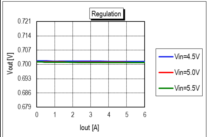
Vout vs. Line Voltage and Load Current @ +25degC. (Vout = 0.7V)
