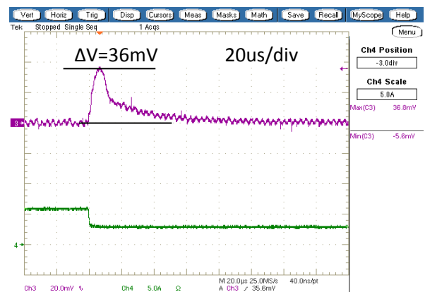
Step Load Transient Response (Vin=12V, Vout=1.0V, Cload=400uF, Iout=3A to 6A, 2.5A/us) Trace 3=Vout, 20 mV/div, Trace 4=Iout, 5A/div.
