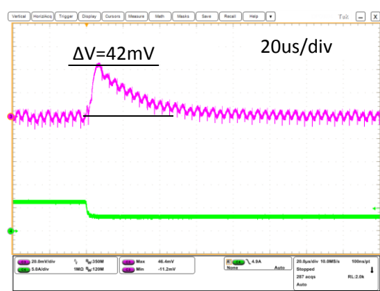
Step Load Transient Response (Vin=5.0V, Vout=0.7V, Cload=400uF, Iout=3A to 6A, 2.5A/us) Trace 3=Vout, 20 mV/div, Trace 4=Iout, 5A/div.
