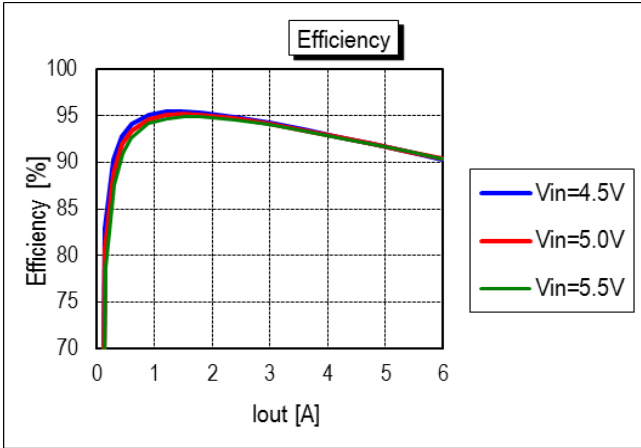
Efficiency vs. Line Voltage and Load Current @ +25degC. (Vout = 1.8V)
