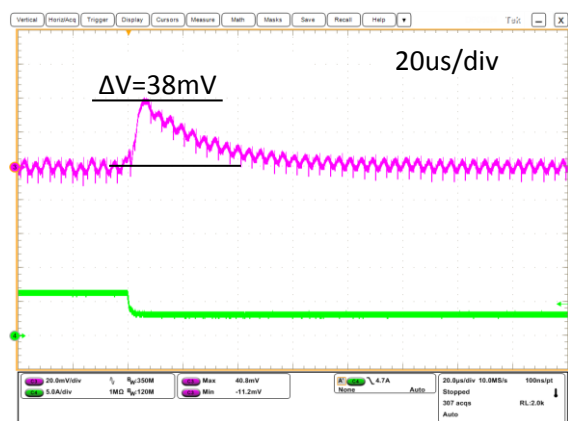
Step Load Transient Response (Vin=5.0V, Vout=1.8V, Cload=400uF, Iout=3A to 6A, 2.5A/us) Trace 3=Vout, 20 mV/div, Trace 4=Iout, 5A/div.
