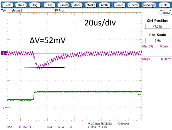
Step Load Transient Response (Vin=12V, Vout=3.3V, Cload=400uF, Iout=3A to 6A, 2.5A/us) Trace 3=Vout, 50 mV/div, Trace 4=Iout, 5A/div.
