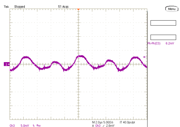
Output Ripple and Noise (Vin=5.0V, Vout=0.7V, Iout=6A, Cload=400uF, ScopeBW=20MHz)
