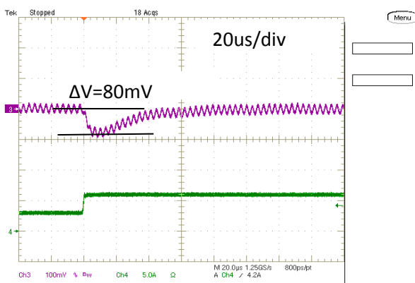
Step Load Transient Response (Vin=12V, Vout=5.0V, Cload=400uF, Iout=3A to 6A, 2.5A/us) Trace 3=Vout, 100 mV/div, Trace 4=Iout, 5A/div.
