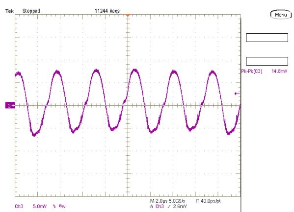
Output Ripple and Noise (Vin=12V, Vout=3.3V, Iout=6A, Cload=400uF, ScopeBW=20MHz)
