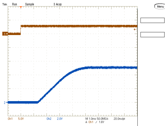
On/Off Enable Delay (Vin=12V, Vout=5.0V, Iout=6A, Cload=400uF) Trace1=Enable, Trace2=Vout, 1 ms/div
