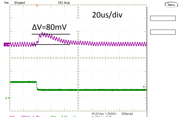
Step Load Transient Response (Vin=12V, Vout=5.0V, Cload=400uF, Iout=3A to 6A, 2.5A/us) Trace 3=Vout, 100 mV/div, Trace 4=Iout, 5A/div.
