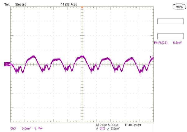
Output Ripple and Noise (Vin=12V, Vout=1.0V, Iout=20A, Cload=400uF, ScopeBW=20MHz)
