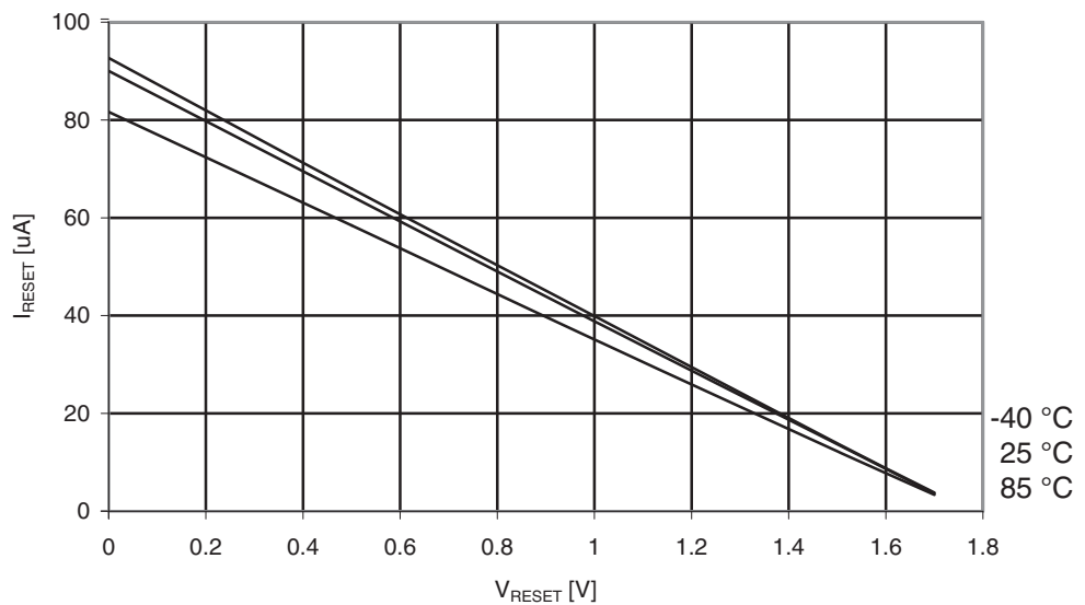
Figure 31-18. Reset Pull-up Resistor Current vs. Reset Pin Voltage V_{CC} = 1.8V
