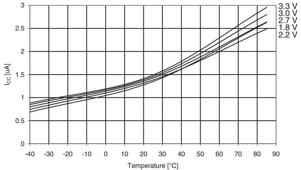
Figure 31-17. Power-save Supply Current vs. Temperature With WDT, sampled BOD and RTC from ULP enabled
