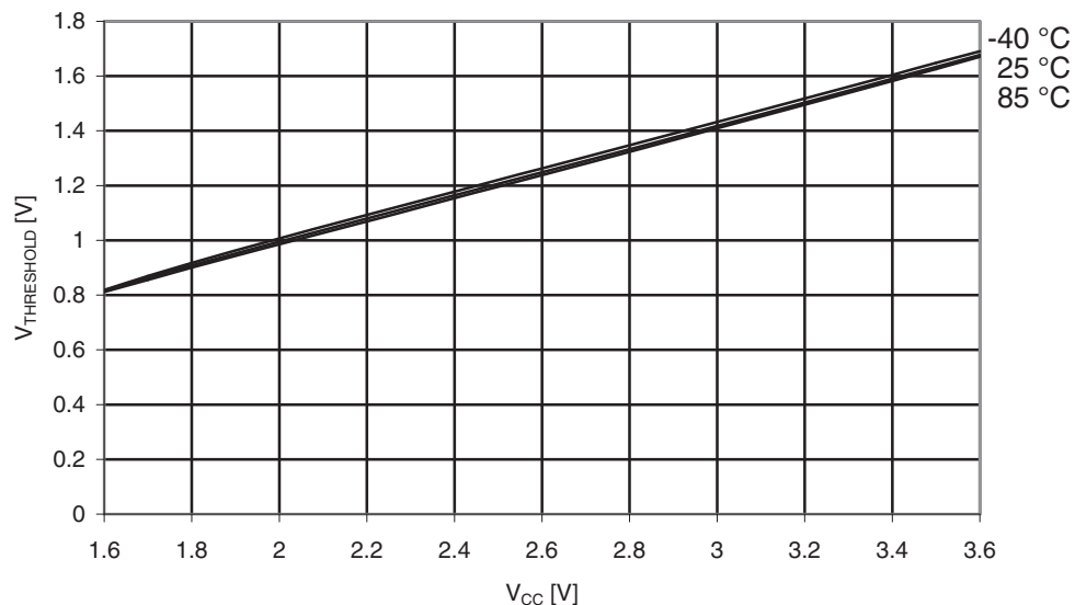
Figure 31-31. Reset Input Threshold Voltage vs. V_{CC} V_{IL} - I/O Pin Read as "0"
