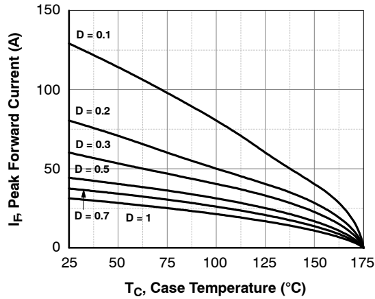
Figure 3. Current Derating
