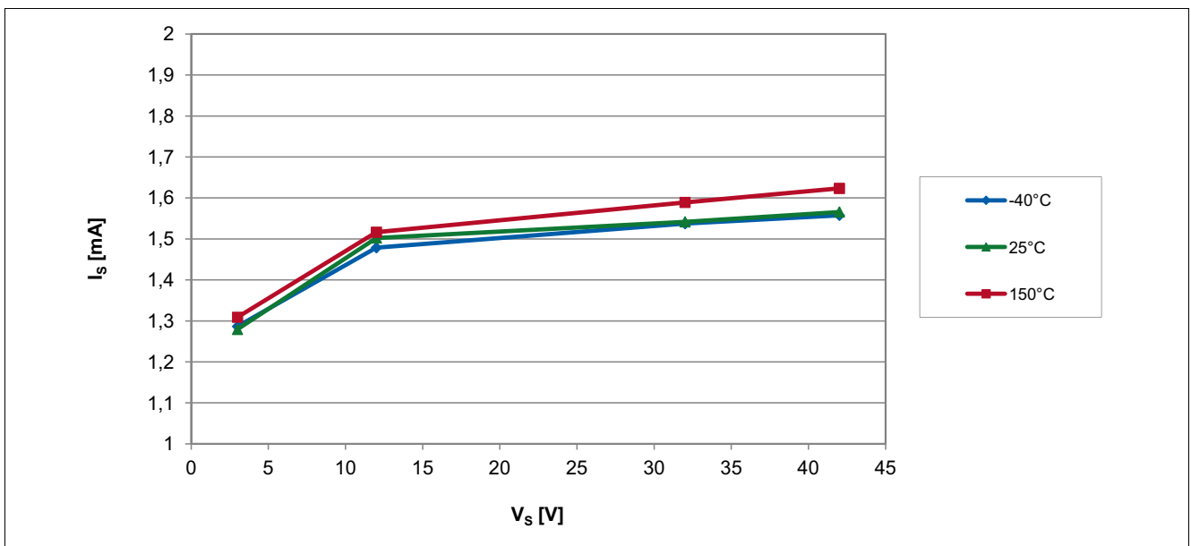
Figure 6-4 Supply Current of the TLV4961-1M over Supply Voltage
