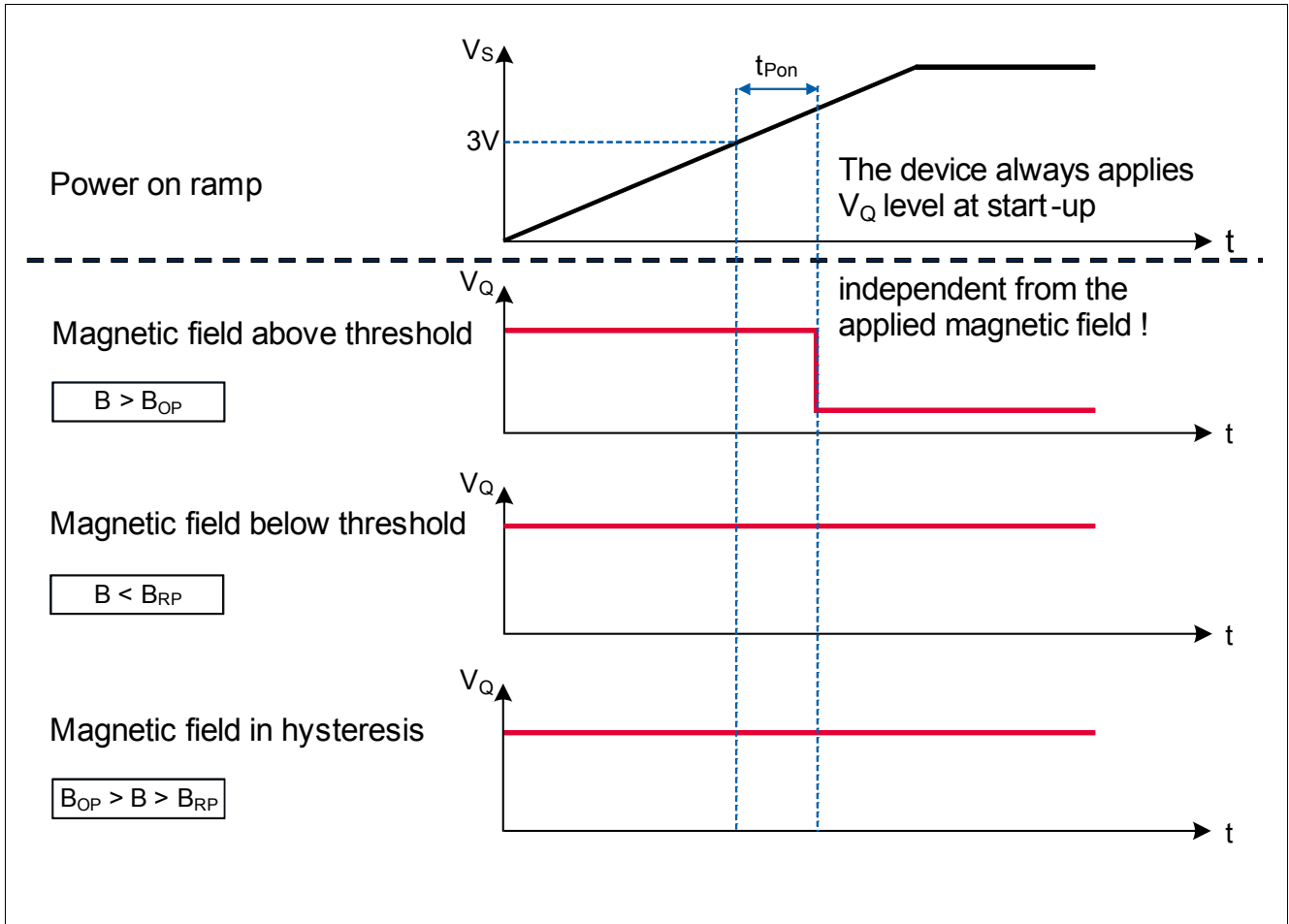
Figure 2-5 Illustration of the start-up behavior of the TLV4961-1M
