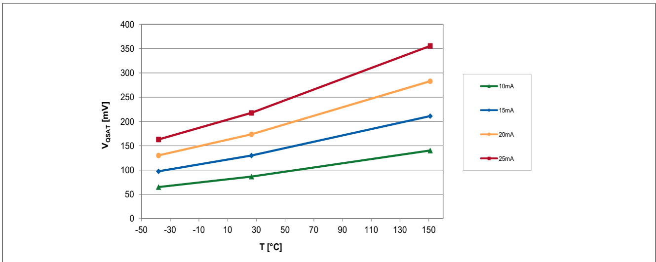
Figure 6-12 Saturation Voltage of the TLV4961-1M over Temperature
