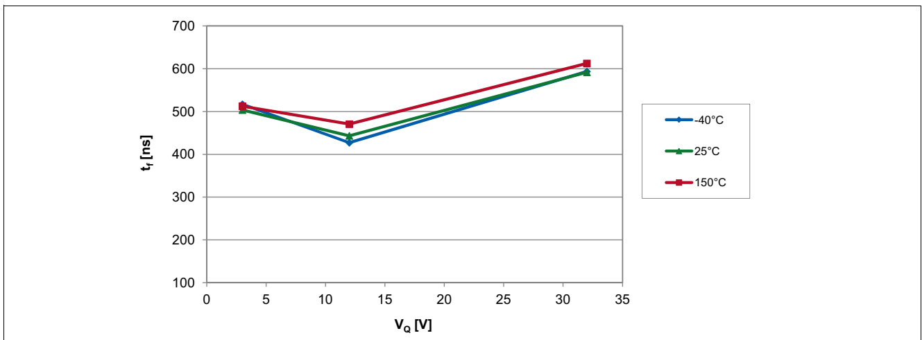
Figure 6-10 Output Rise Time of the TLV4961-1M over applied Pull-up Voltage
