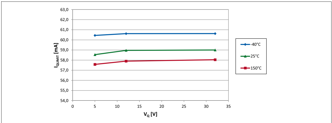
Figure 6-6 Output Current Limit of the TLV4961-1M over applied Pull-up Voltage
