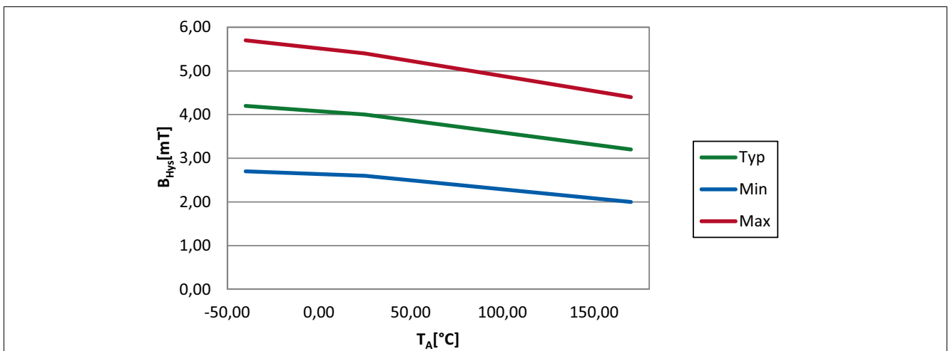
Figure 5-3 Hysteresis ( B_{Hys} ) of the TLV4961-1M over Temperature
