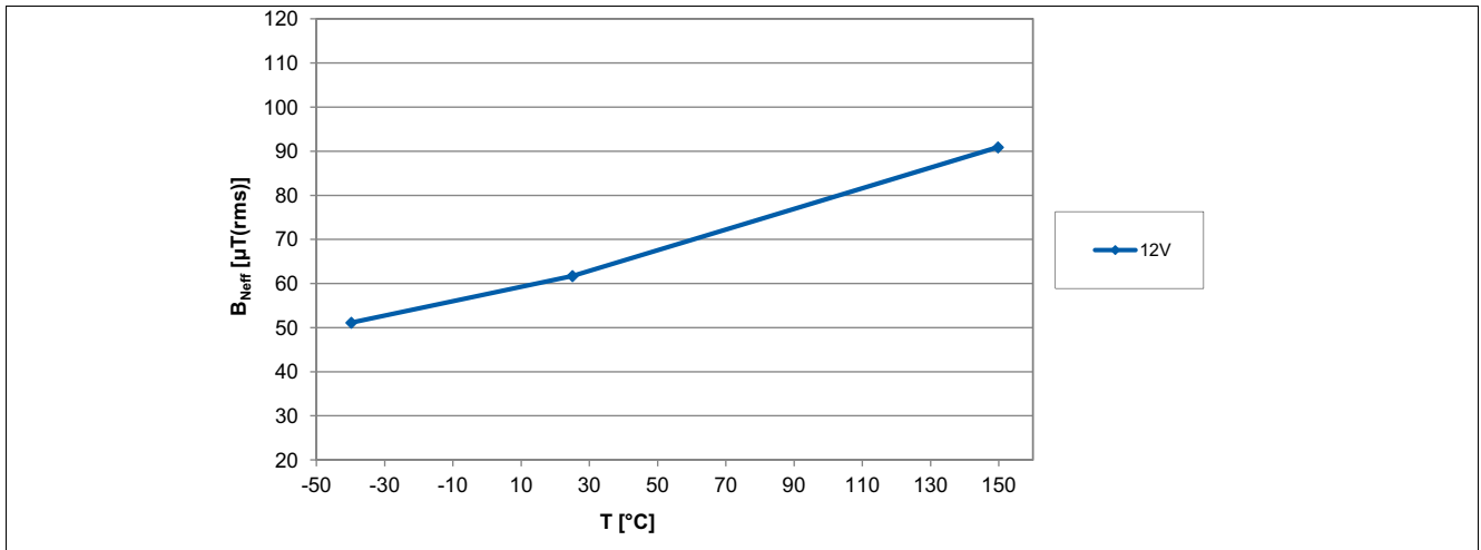
Figure 6-14 Effective Noise of the TLV4961-1M Thresholds over Temperature
