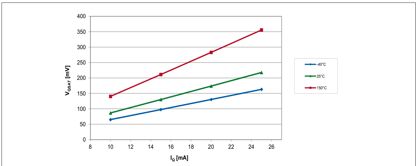
Figure 6-13 Saturation Voltage of the TLV4961-1M over Output Current
