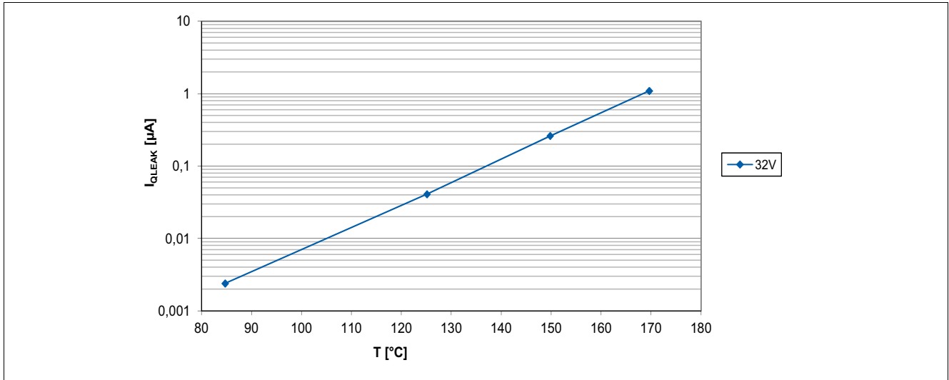
Figure 6-11 Output Leakage Current of the TLV4961-1M over Temperature
