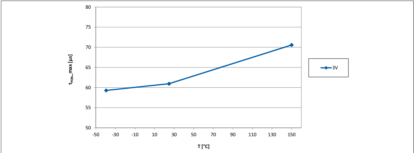
Figure 6-1 Power On Time t_{PON} of the TLV4961-1M over Temperature
