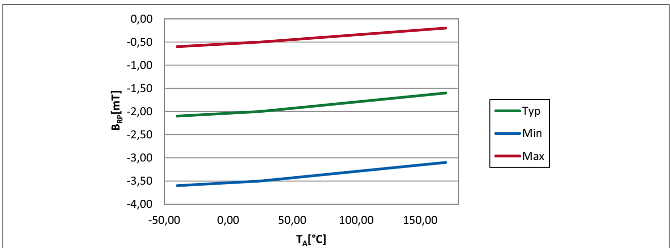
Figure 5-2 Release Point ( B_{RP} ) of the TLV4961-1M over Temperature
