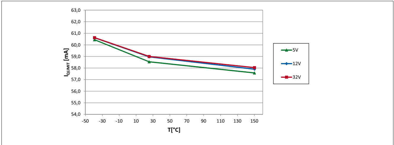
Figure 6-5 Output Current Limit of the TLV4961-1M over Temperature
