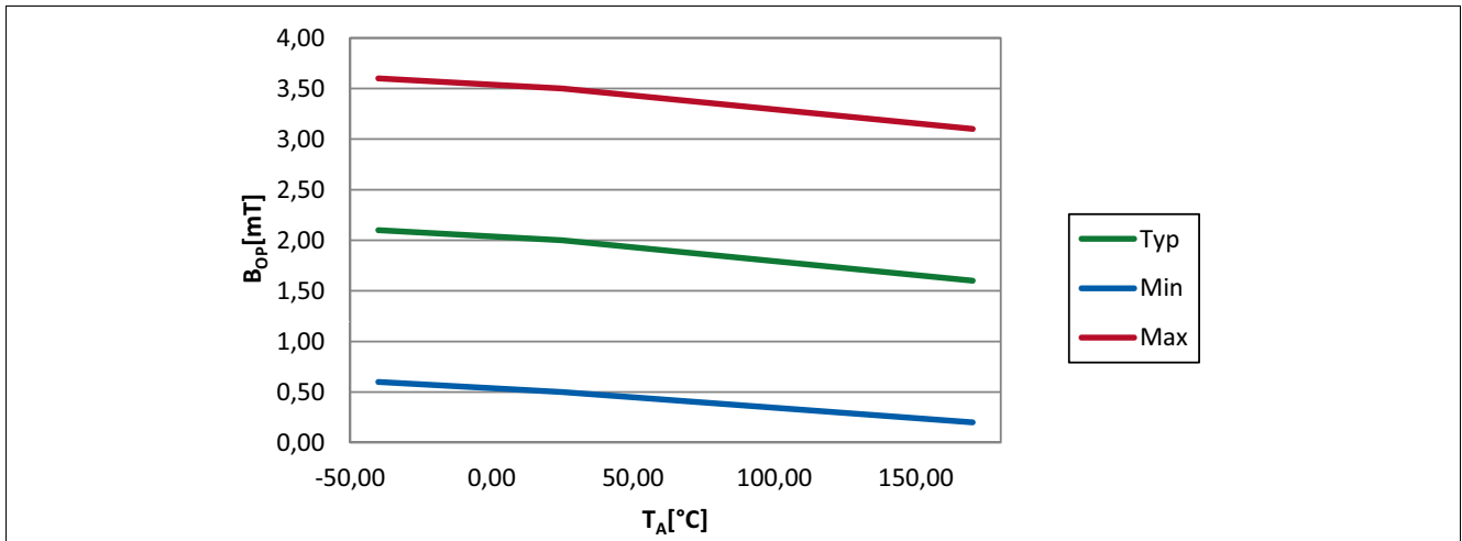
Figure 5-1 Operating Point ( B_{OP} ) of the TLV4961-1M over Temperature
