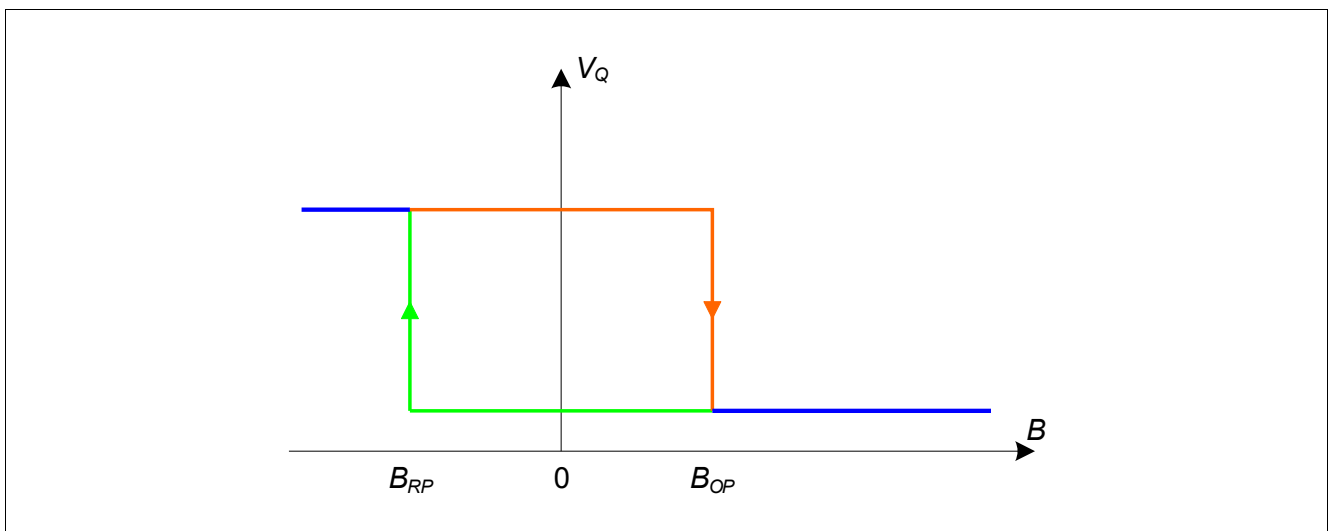
Figure 2-4 Output Signal TLV4961-1M
