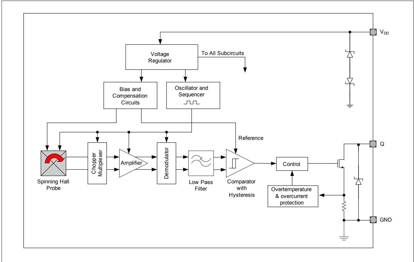
Figure 2-2 Functional Block Diagram TLV4961-1M
