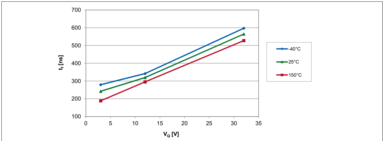
Figure 6-8 Output Fall Time of the TLV4961-1M over applied Pull-up Voltage
