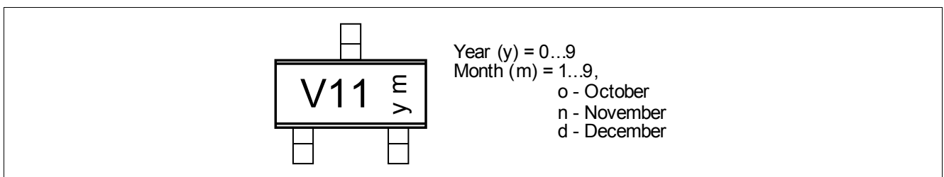
Figure 4-5 Marking of TLV4961-1M
