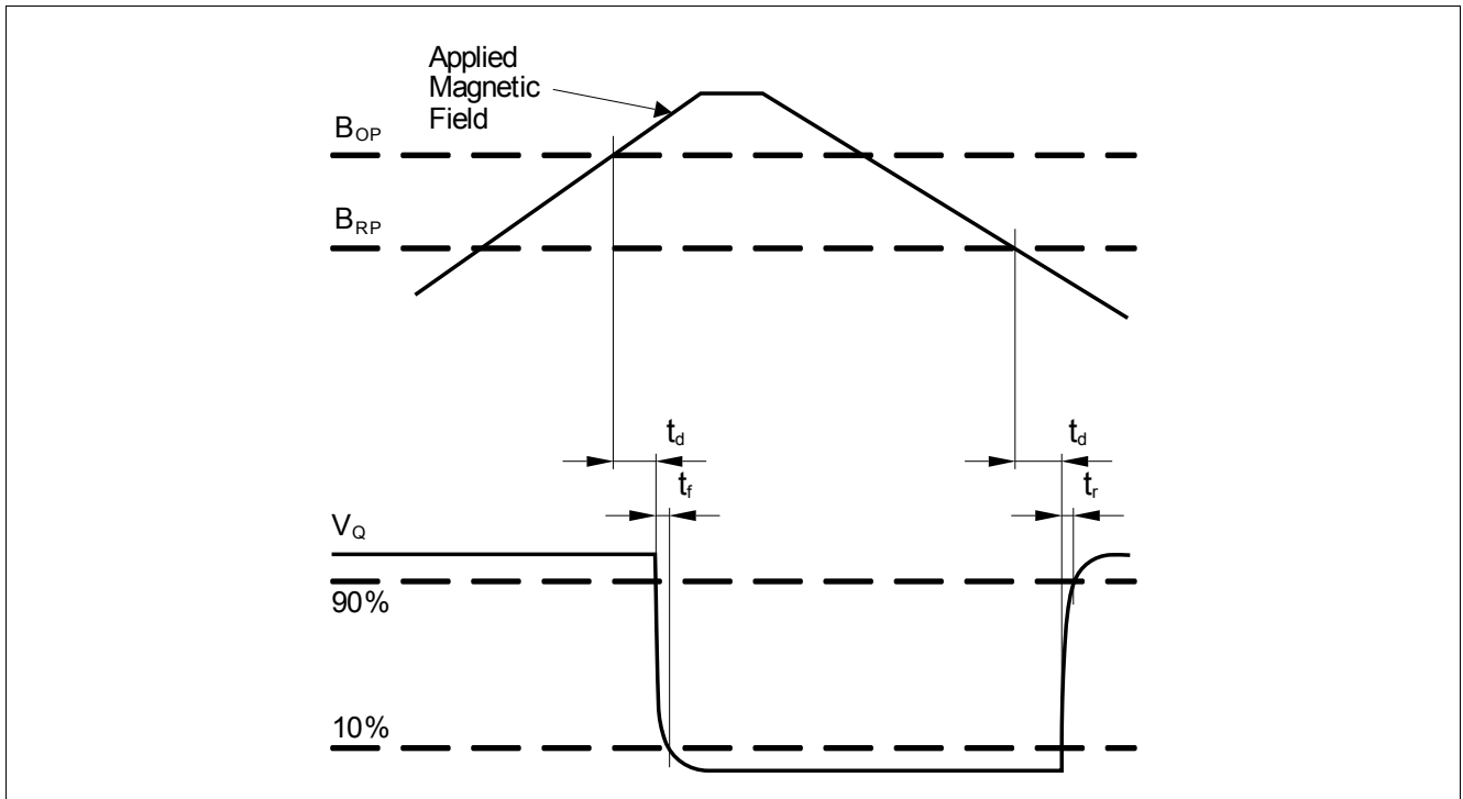
Figure 2-3 Timing Diagram TLV4961-1M
