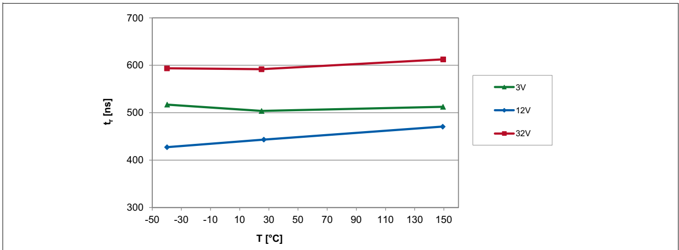
Figure 6-9 Output Rise Time of the TLV4961-1M over Temperature
