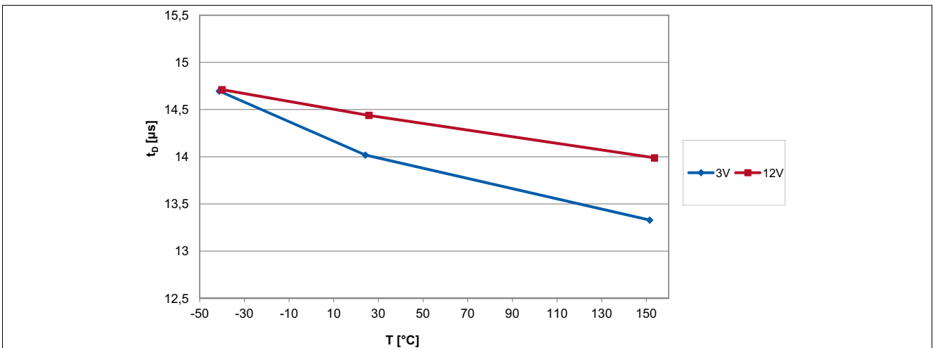
Figure 6-2 Signal Delay Time of the TLV4961-1M over Temperature
