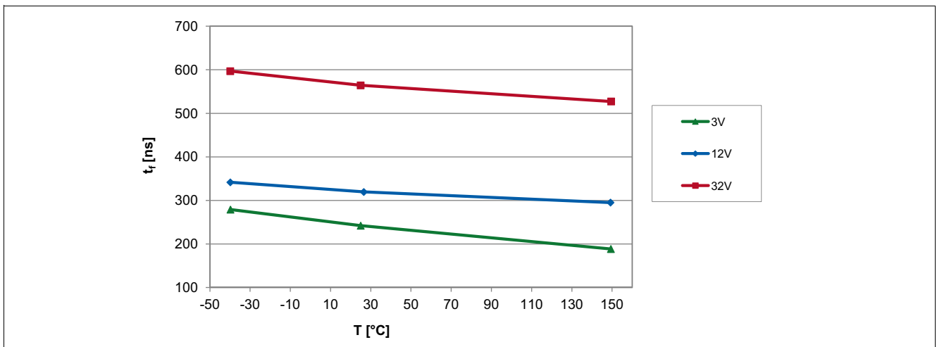
Figure 6-7 Output Fall Time of the TLV4961-1M over Temperature
