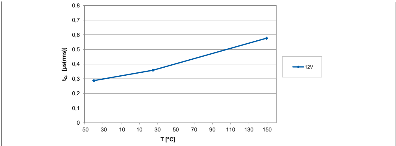
Figure 6-15 Output Signal Jitter of the TLV4961-1M over Temperature
