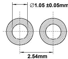
Figure 9: Recommended PCB Through Hole Size
