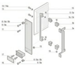
Item 9a, 3 U front panel mounting
