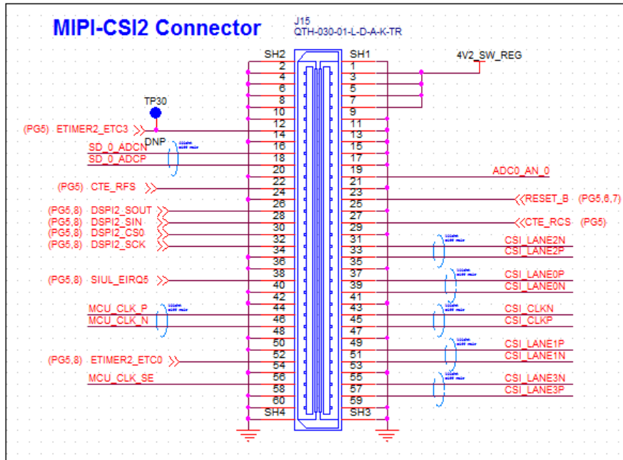
Figure 19. MIPI-CSI2 connector pinout
