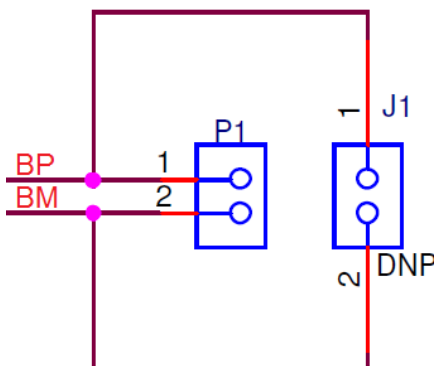
Figure 11. FlexRAY alternative connector pin-outs
