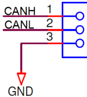
Figure 6. CAN 3pin header interface connector
