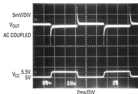
Line Transient Response (See Figure 2, I_L = 10\text{mA} )
