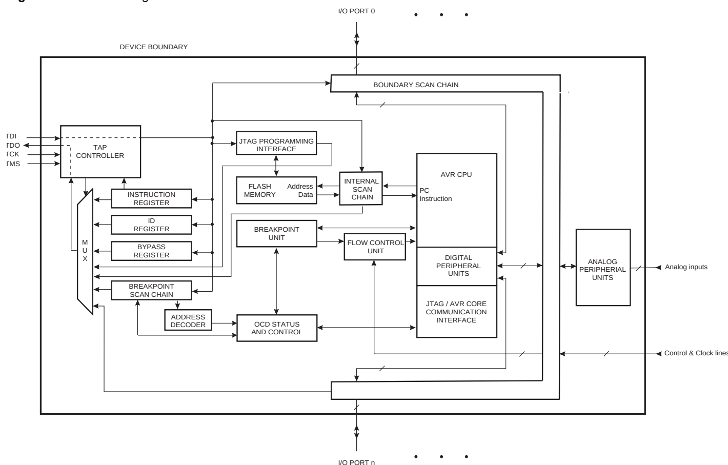
Figure 24-1. Block diagram.
