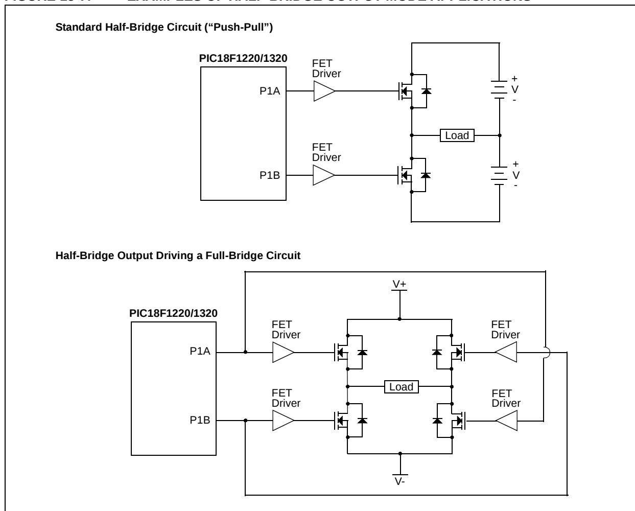
FIGURE 15-7: EXAMPLES OF HALF-BRIDGE OUTPUT MODE APPLICATIONS
