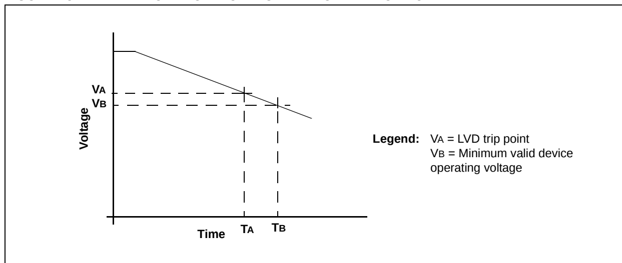
FIGURE 18-1: TYPICAL LOW-VOLTAGE DETECT APPLICATION
