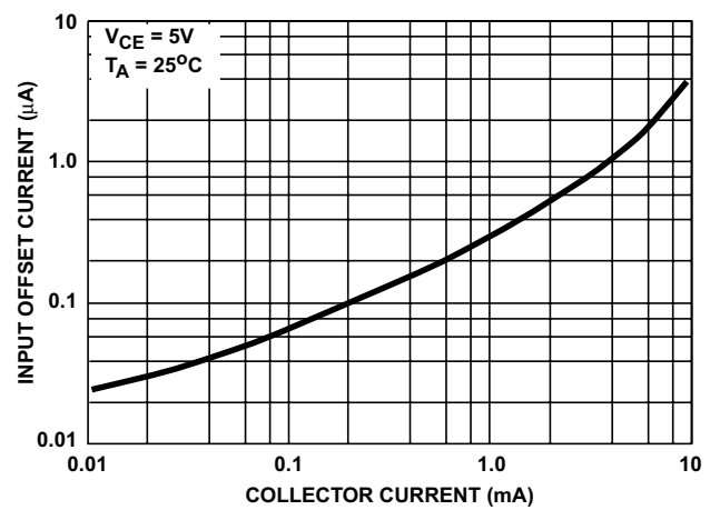
FIGURE 8. I_O vs I_C FOR Q_1 AND Q_2
