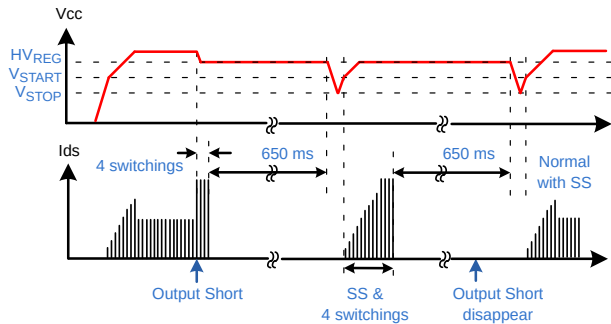
Figure 24. AOCPS Waveform
