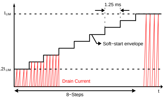
Figure 27. Internal Soft-Start
