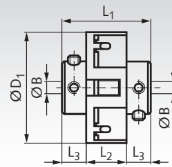
Set-screw style
