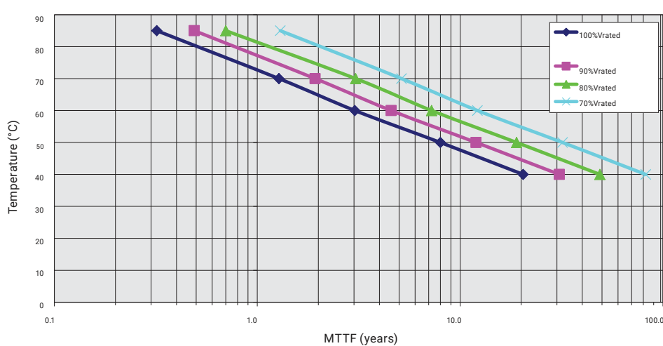
Expected Lifetime at Various Voltages SCM Series, 4.6V/4.2V, 5.0V/4.6V, 6.4V, 7.6V/6.9V Rated
