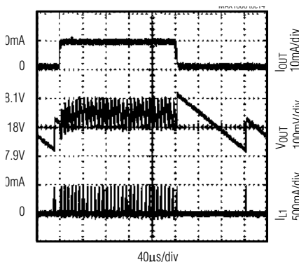
V_{OUT} = 18V , I_{OUT} = 1mA TO 10mA V_{CC} = 3.3V , V_{IN} = V_{BATT} = 3.6V
