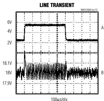
A: V_{BATT} = V_{CC} = 2.4V TO 5.5V , 2V/div B: V_{OUT} = 18V , R_{OUT} = 3.6k\Omega , 100mV/div
