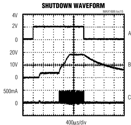
A: \overline{SHDN} , 2V/div B: V_{OUT} , 10V/div , R_{OUT} = 1.8k\Omega C: I_{L1} , 500mA/div
