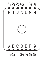
3 POLES
