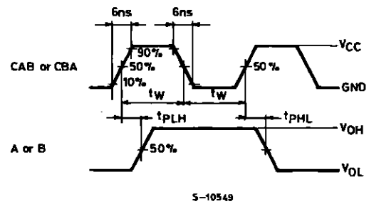
WAVEFORM 2
