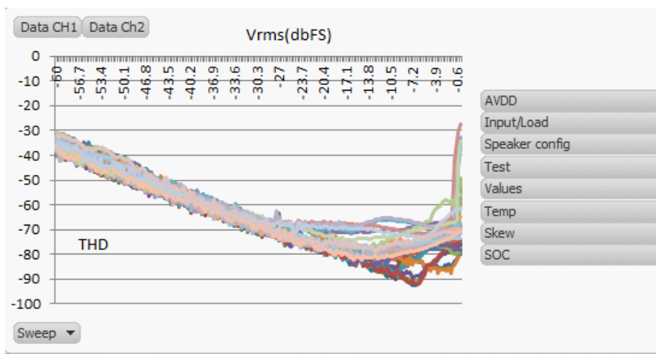
Figure 3-10. DAC Signal Quality – THD (Single-ended)
