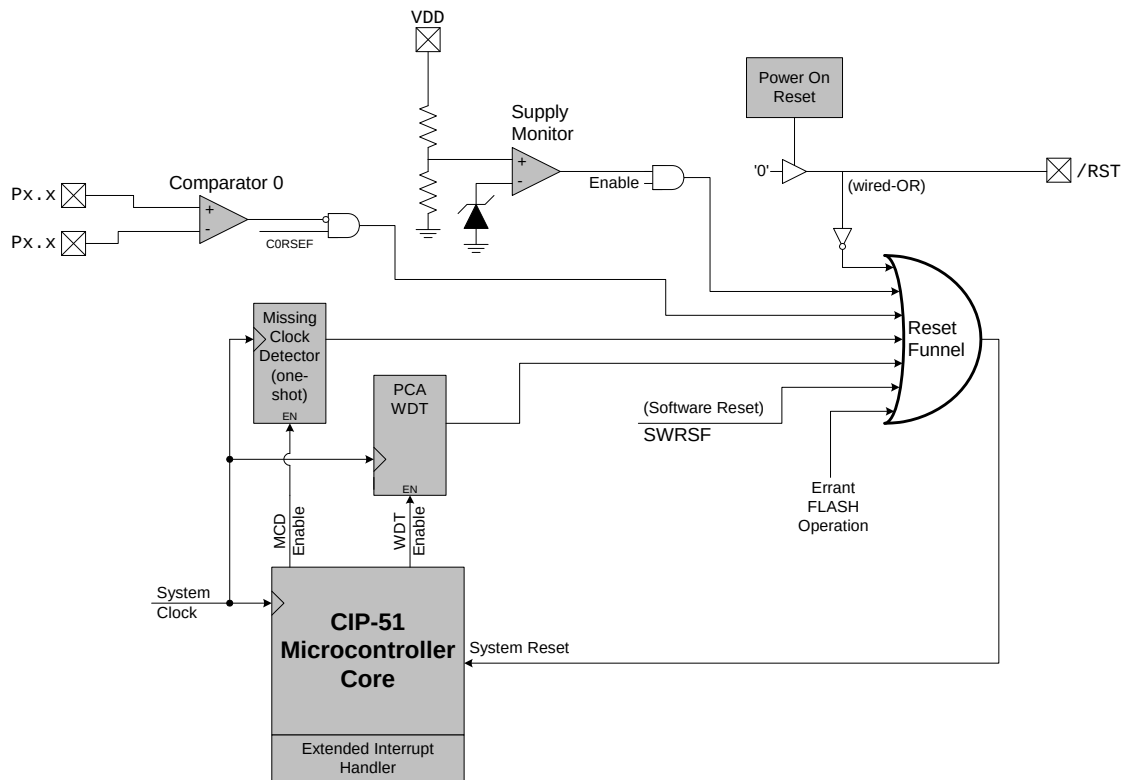
Figure 17.1. Reset Sources
