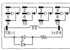
4PDT
