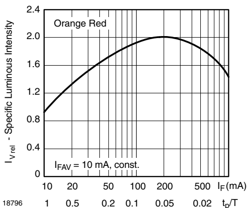
Fig. 5 - Rel. Lumin. Intensity vs. Forward Current/Duty Cycle
