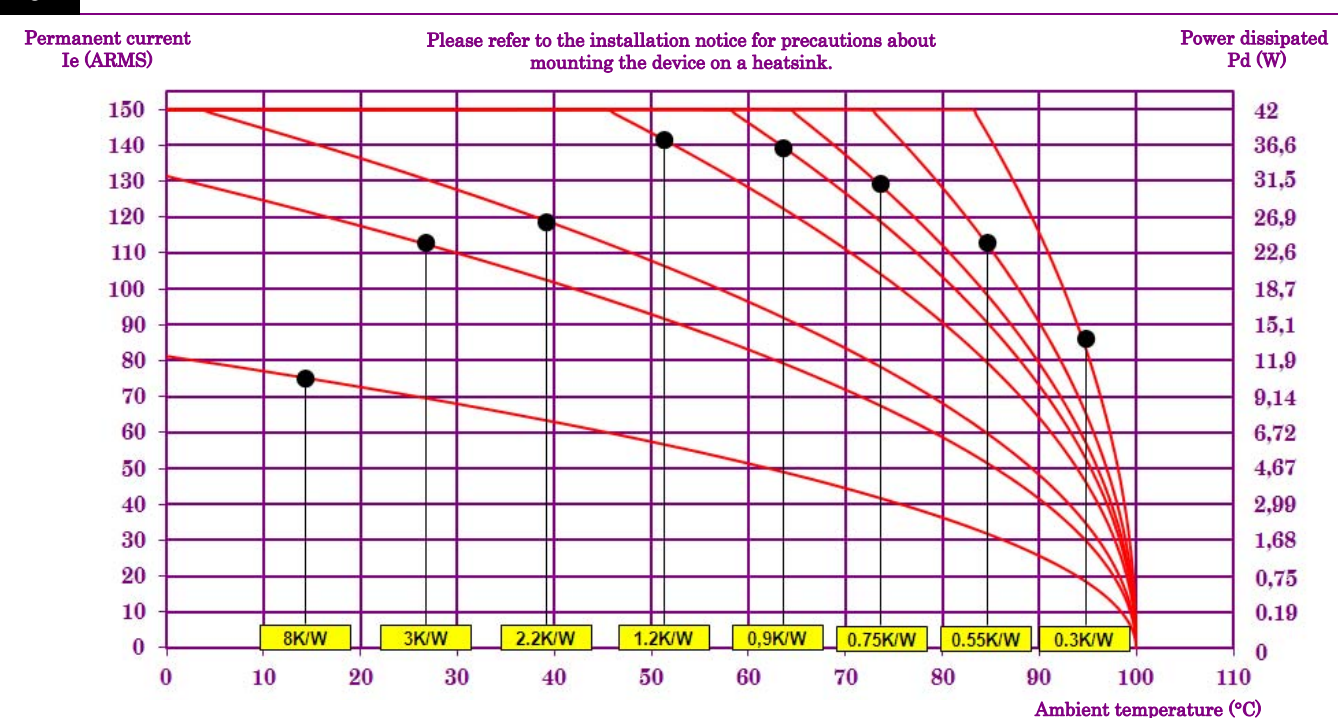
Fig. 9 POWER DISSIPATED AND LOAD CURRENT LIMIT VS TEMPERATURE
