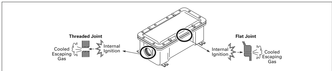
Figure 47-157. Explosion Proof Enclosure
