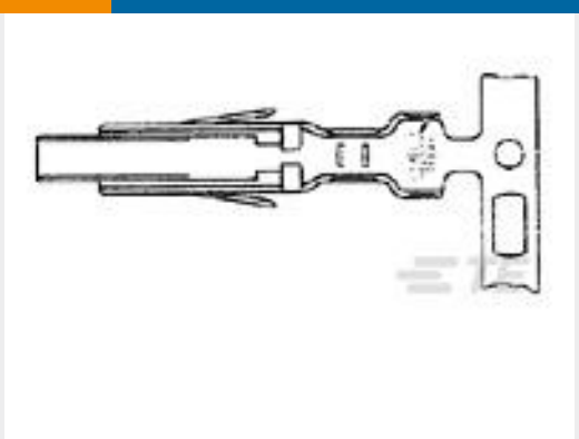
TE Part #170485-1 DRAWER CONN LP
