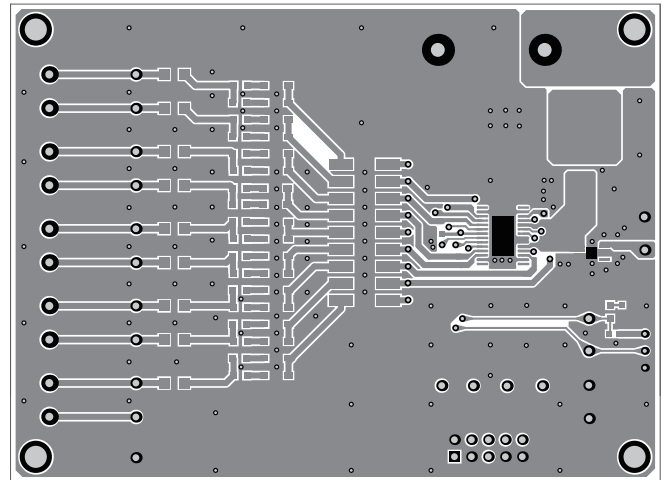
Figure 2: Top Layer
