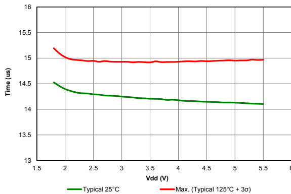
Figure 39-54. Wake From Sleep, VREGPM = 'b0x, HFINTOSC = 16MHz
