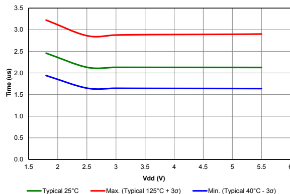
Figure 39-1. ADC RC Oscillator Period vs. Vdd
