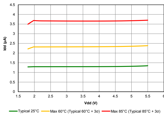
Figure 39-47. I_{PD} , WATCH DOG TIMER (WDT)
