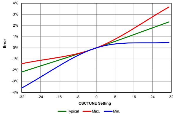
Figure 39-63. OSCTUNE Frequency Range (Normalized to Center Frequency)
