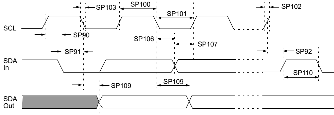
Figure 38-20. I 2 C Bus Data Timing
