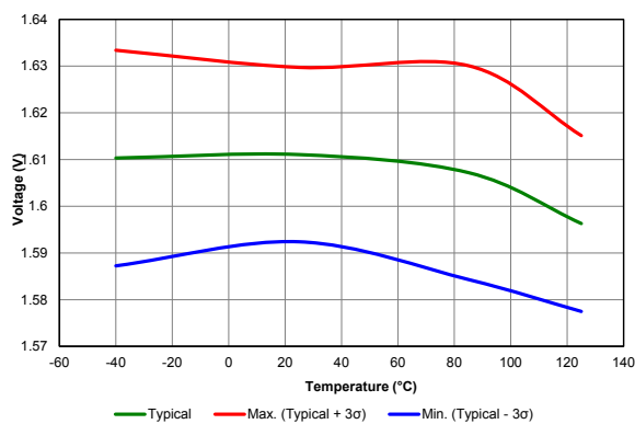
Figure 39-64. POR RELEASE VOLTAGE (VREGPM = 'b1x)
