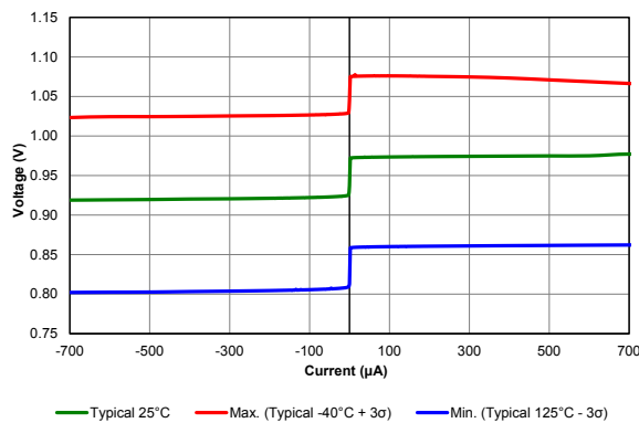
Figure 39-86. ZCD Behavior, V DD = 5.5V
