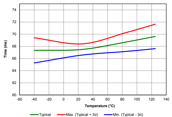
Figure 39-68. PWRT PERIOD vs. Temperature ( V_{DD} = 3.0V )
