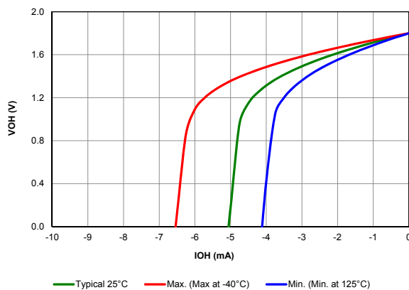
Figure 39-79. VOH vs. IOH OVER TEMPERATURE, V_{DD} = 1.8V
