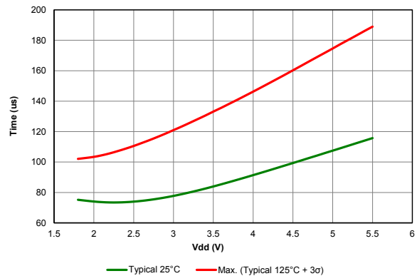
Figure 39-55. Wake From Sleep, VREGPM = 'b10, HFINTOSC = 16MHz
