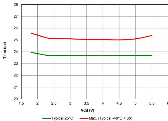
Figure 39-54. Wake From Sleep, VREGPM = 'b0x, HFINTOSC = 16MHz
