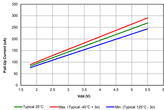
Figure 39-85. Weak Pull Up Current
