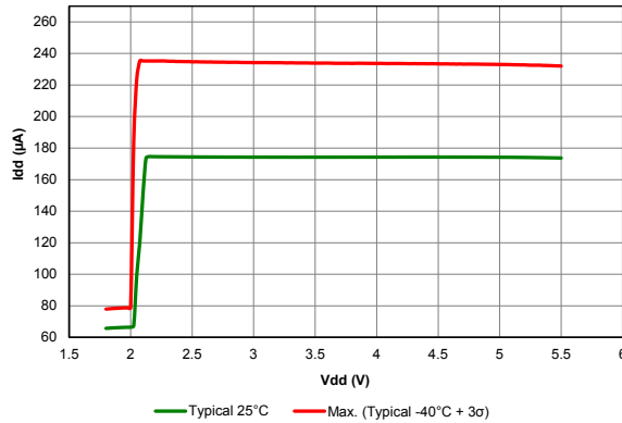
Figure 39-51. I_{PD} BASE (VREGPM='b00)
