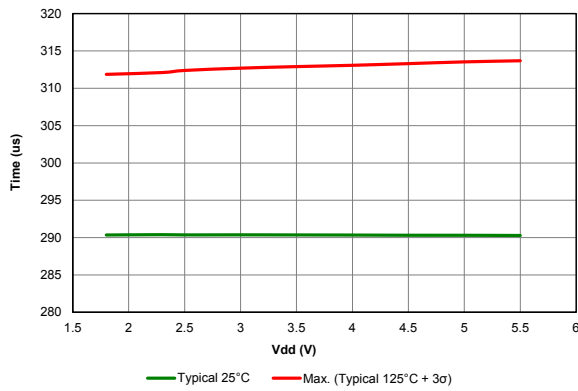
Figure 39-56. Wake From Sleep, VREGPM = 'b01
