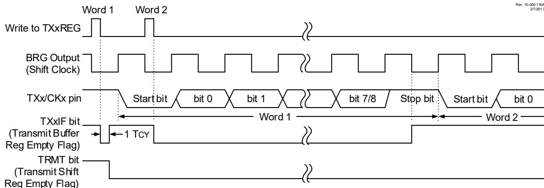
Figure 27-4. Asynchronous Transmission (Back-to-Back)
