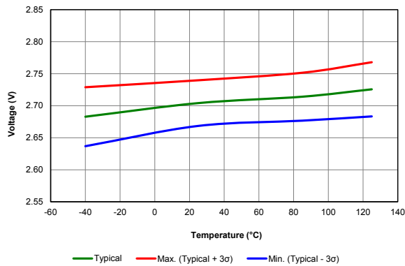
Figure 39-16. BROWN-OUT RESET VOLTAGE, TRIP POINT (BORV = 10 )
