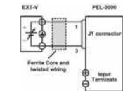
External Voltage Connection
