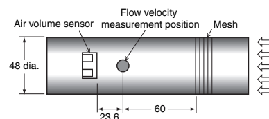
Figure 1: Wind Tunnel
