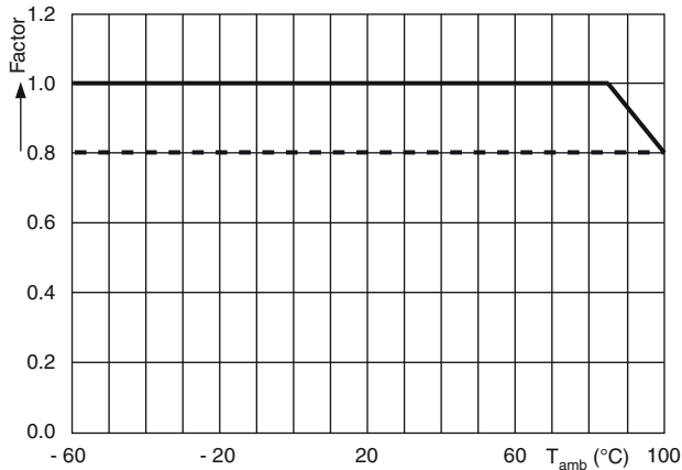
Max. DC and AC voltage as a function of temperature for voltage 63 V
