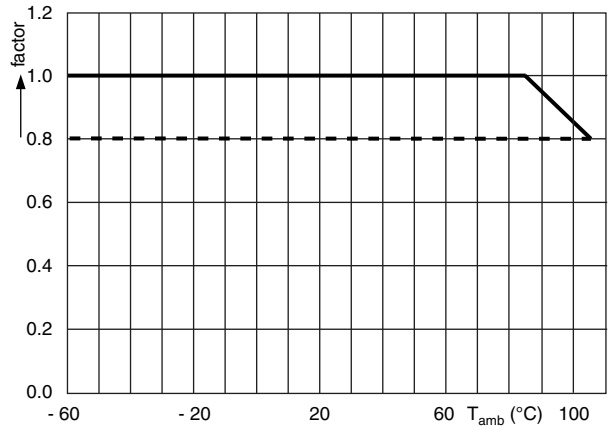
Max. DC and AC voltage as a function of temperature for voltages > 63 V
