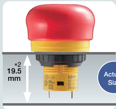
*2: Solder terminal. Solder/tab terminal: 23.9mm
