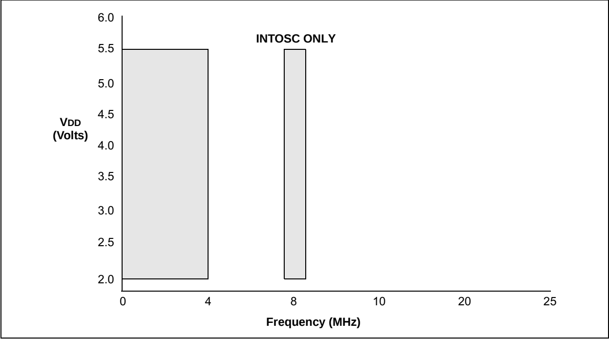
FIGURE 11-1: PIC12F519 VOLTAGE-FREQUENCY GRAPH, -40°C ≤ TA ≤ +125°C
