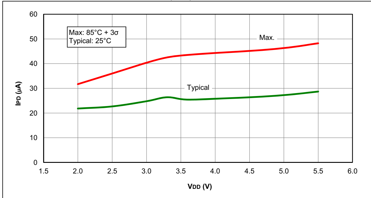
FIGURE 31-37: I_{PD} , BROWN-OUT RESET (BOR), PIC12F1822 AND PIC16F1823 ONLY
