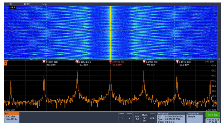
Spectrogram display illustrates slowly moving RF phenomena. As shown here, a signal that has multiple peaks is being monitored. As the peaks change in both frequency and amplitude over time, the changes are easily seen in the Spectrogram display.
