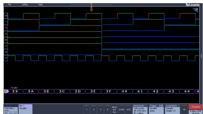
With color-coded digital waveform display, groups are created by simply placing digital channels together on the screen, allowing digital channels to be moved as a group.
