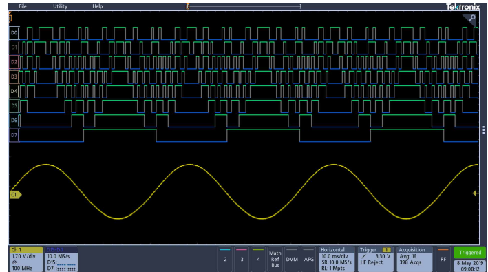
The 3 Series MDO with 3-MSO option is used to simultaneously view analog and digital signals by probing both sides of a D/A converter.
