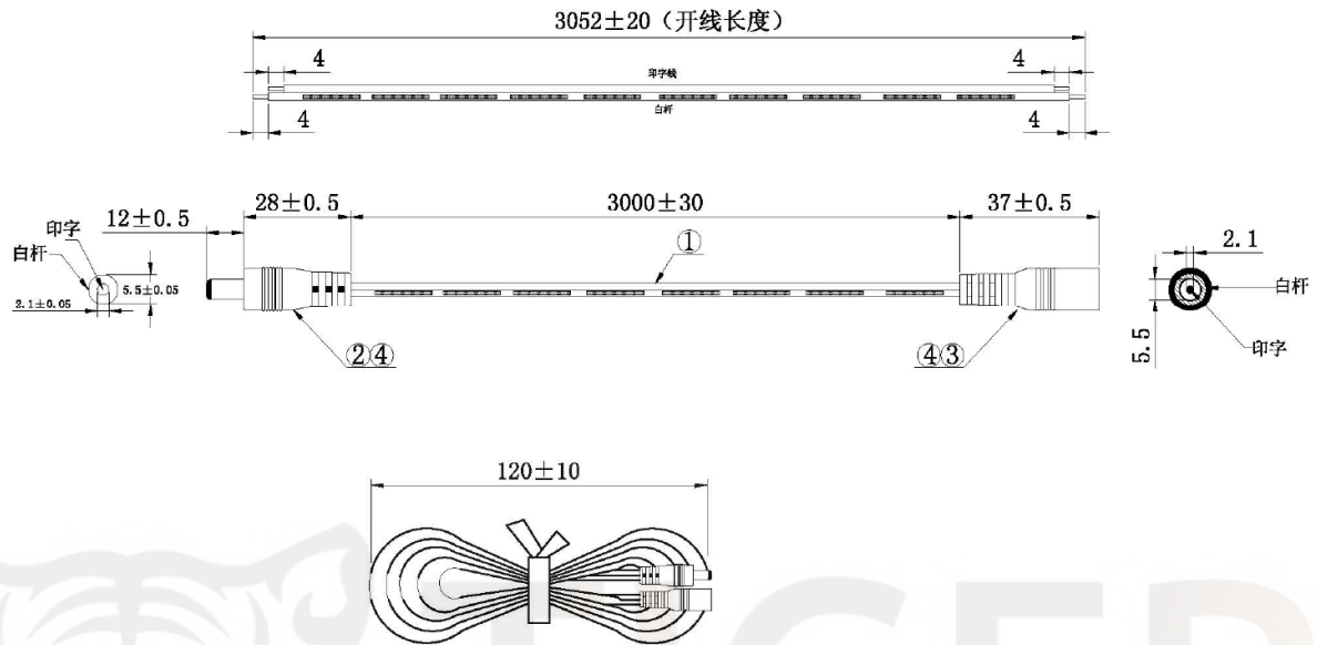
Drawing of TGR-01905 cable
