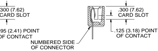
SINGLE ROW CONTACTS READ ONE SIDE OF DAUGHTER BOARD
