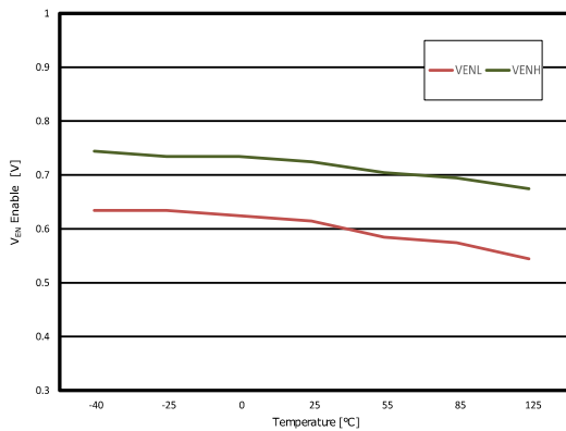
Figure 13: Enable thresholds vs temperature ( I_{OUT} = 1 \text{ mA} )
