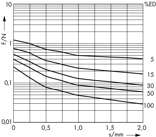
Force vs. Stroke diagramm F = f (s) Force measured when operating in horizontal position, at 90 % rated voltage and with winding at operating temperature stroke s = 0 corresponds to armature in fully home position
