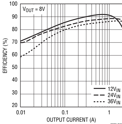
Efficiency (8V OUT )
