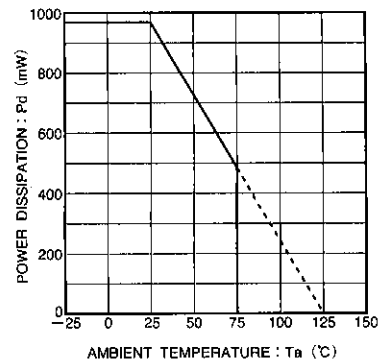
Fig. 6 Power dissipation vs. ambient temperature
