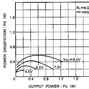
Fig. 5 Power dissipation vs. output power
