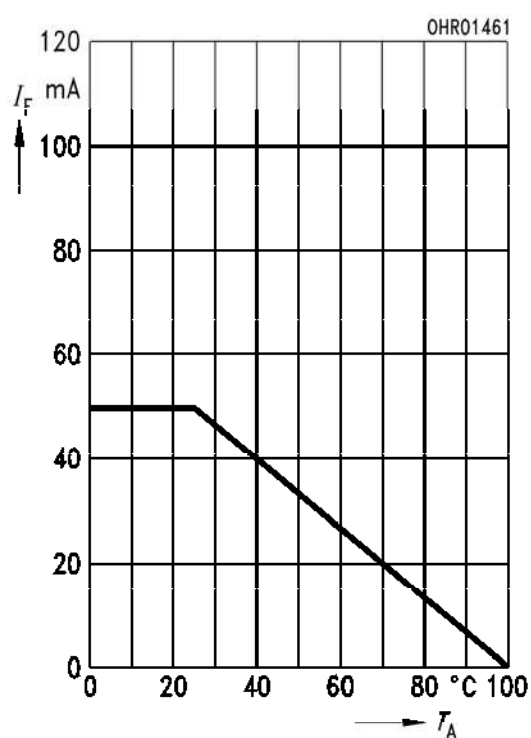
Maximum Permissible Forward Current I_F = f(T_A) , R_{\text{thJA}} = 450 \text{ K/W}
